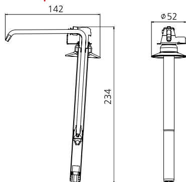
IMP T/TLS 25 Pump
